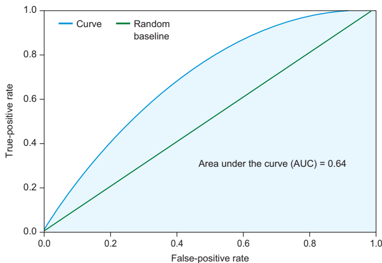
Figure 6.8 The ROC curve of the nonlinear random forest model. The AUC is significantly better: at 0.64, it’s likely that there’s a real signal in the dataset.
